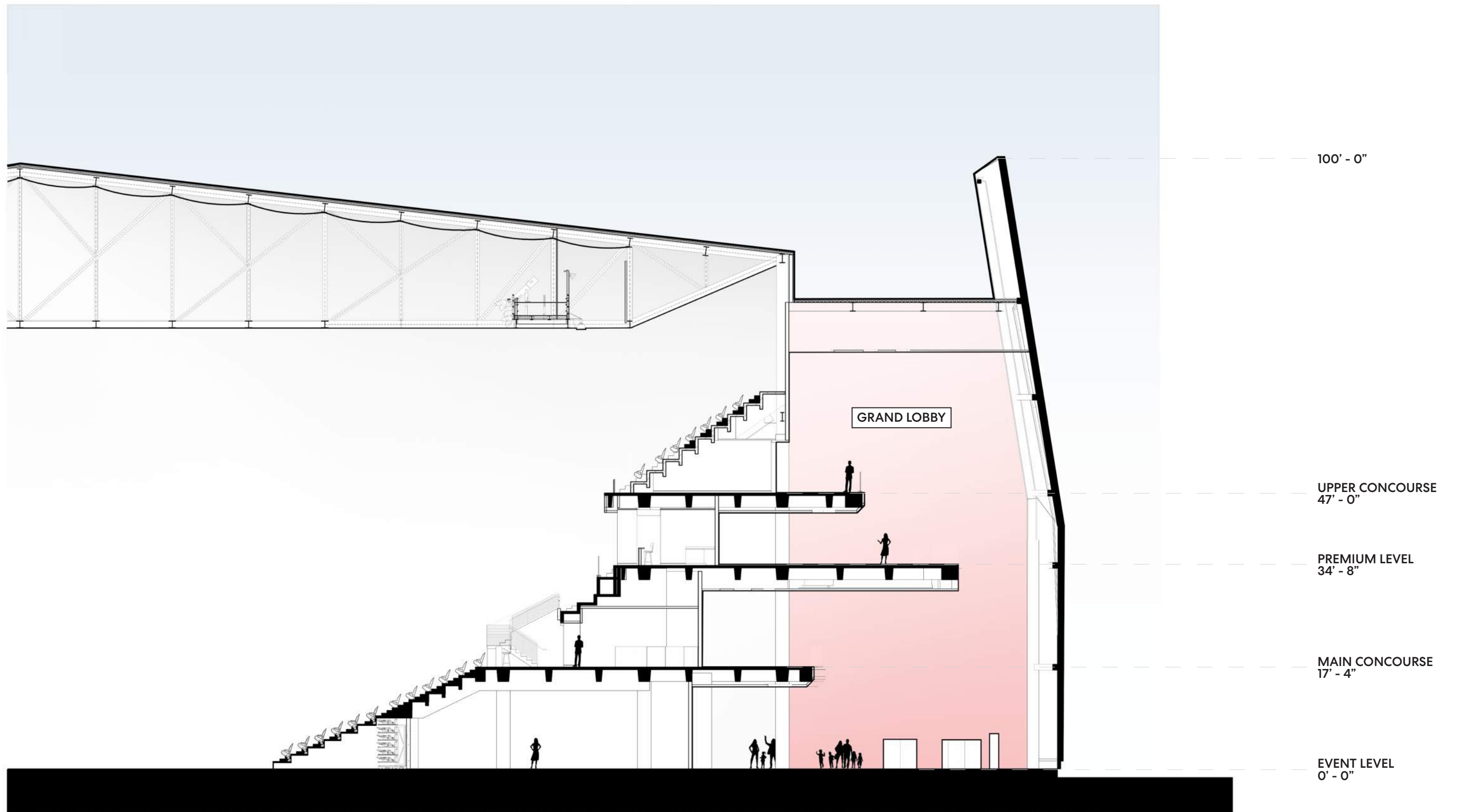
TRANSVERSE SECTION
